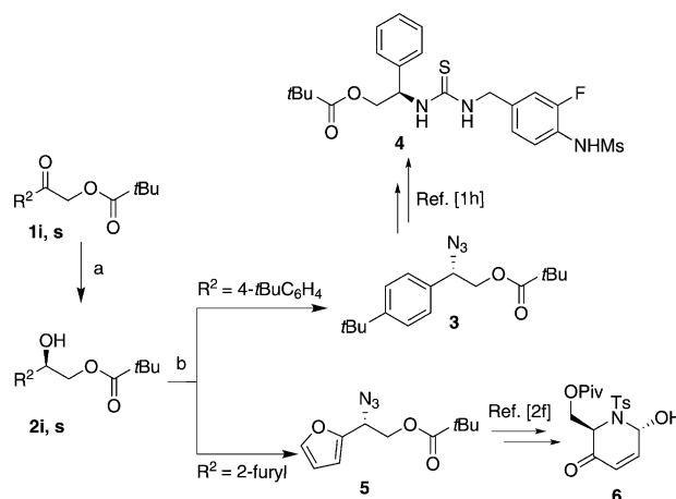
Scheme 1. Reagents and conditions: a) L4 (2.4 mol %) and Pd-(OCOCF 3 ) 2 (2.0 mol %), H 2 (30 bar), EtOH/TFE (> 99 % conversions and 96 %, 97 % ee ); b) DPPA, DBU, toluene (71 % and 77 % yield, 95 % and 92 % ee for 3 and 5 , respectively). DBU = 1,8-diazabicyclo-[5.4.0]undec-7-ene, DPPA = diphenylphosphoryl azide.
